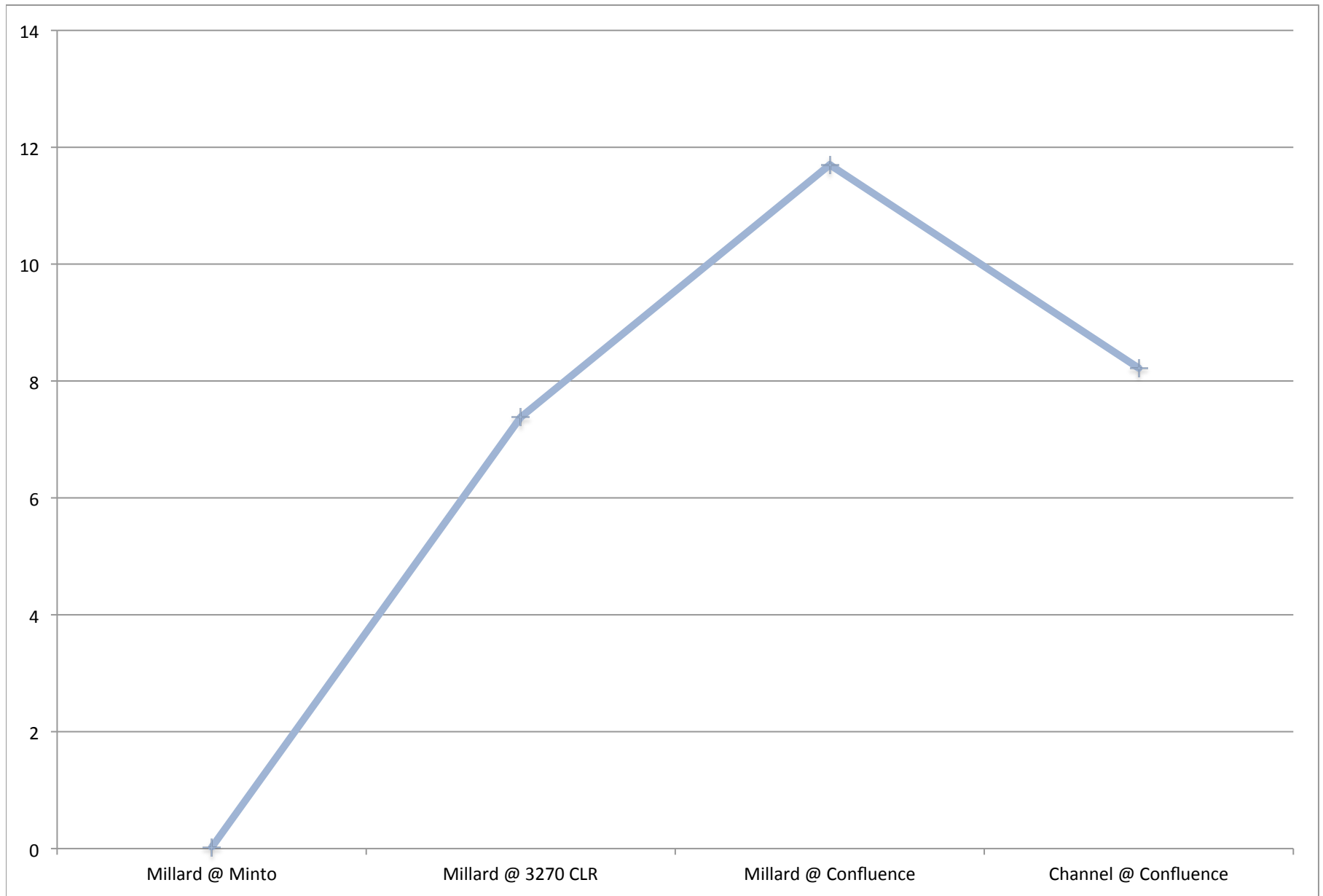
Millard Creek water turbidity 17th Nov 2015
